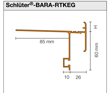
H = 4 / 10 / 15 / 18 / 21 mm
