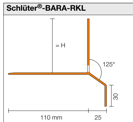
H = 30 / 35 / 40 / 50 / 75 mm
