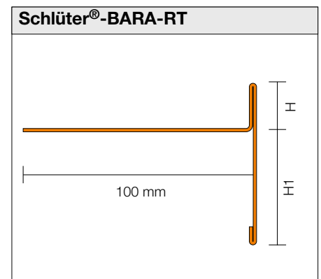
H/H1 = 9/60, 12/16, /12/65, 20/50, 25/40, 30/35 mm
