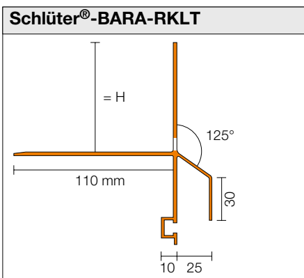
H = 30 / 40 / 50 / 75 mm
